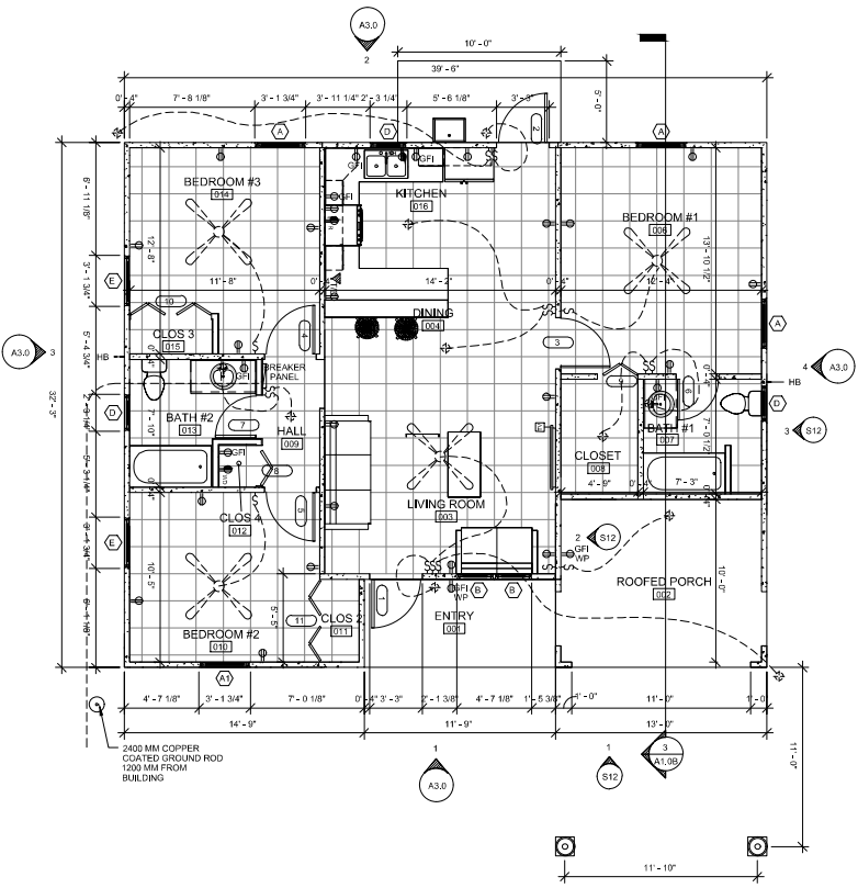
1 FLOOR PLAN - BASE MODEL 1:50
